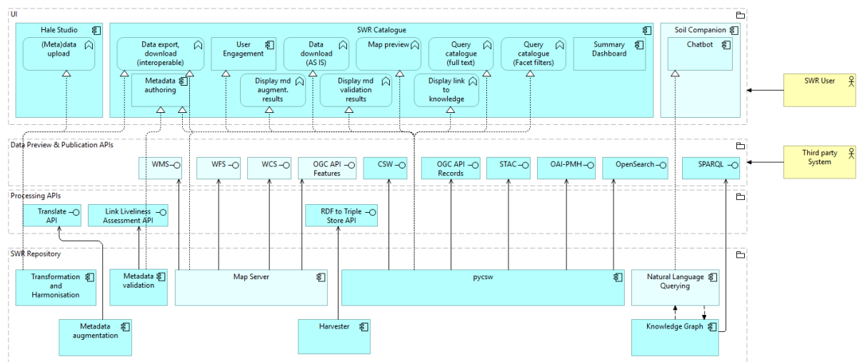
Figure 2: SWR Interfaces (light blue elements are under development and not part of 2 nd prototype)
