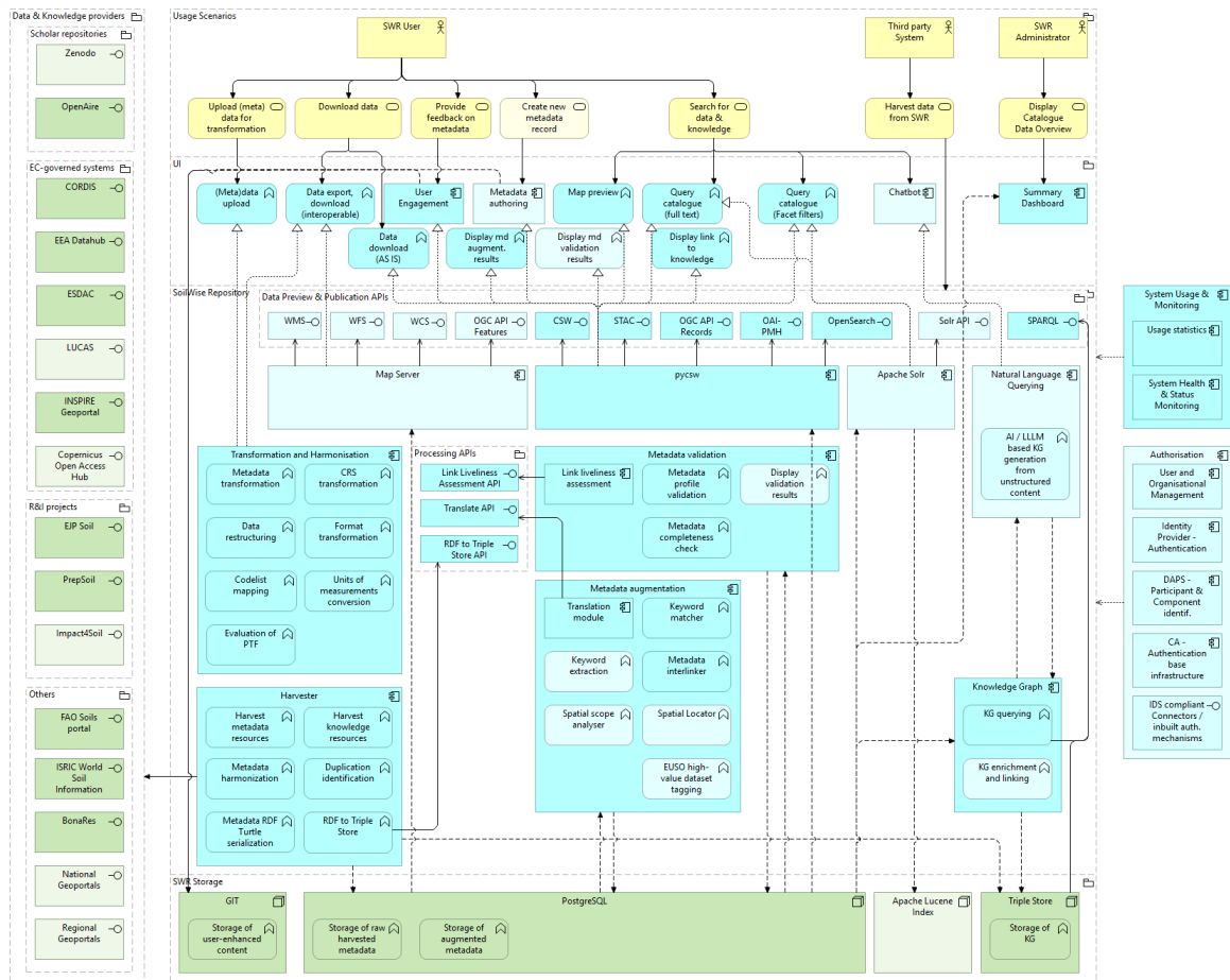
Figure 1: SWR 2 nd prototype architecture (light-colored elements are under development and not part of 2 nd prototype)
